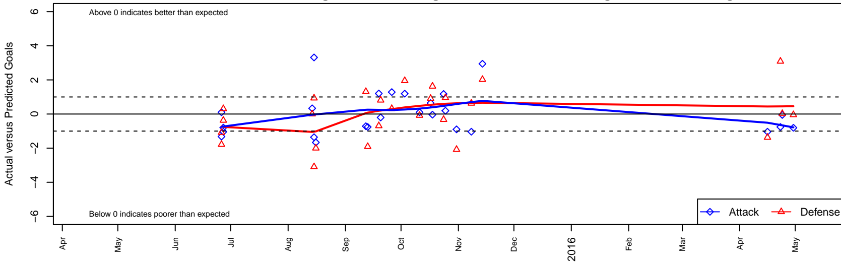
Washington Timbers Red G04 Dots are actual minus expected GF (blue circles) and GA (red triangles). Blue line is smoothed change in attack strength. Red is smoothed change in defense strength.
